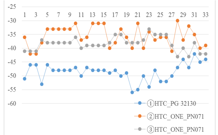
Fig. 2. Comparison of 33 RSSI values received from three smartphones at a 5-second sampling rate
