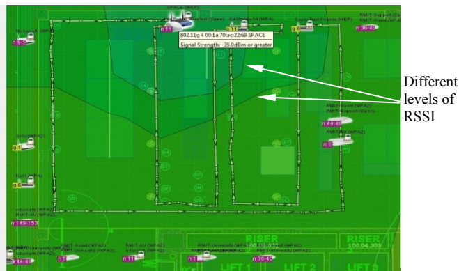
Fig. 1. Map of Wi-Fi signal propagation (tested in the Indoor Positioning Lab, RMIT University)
